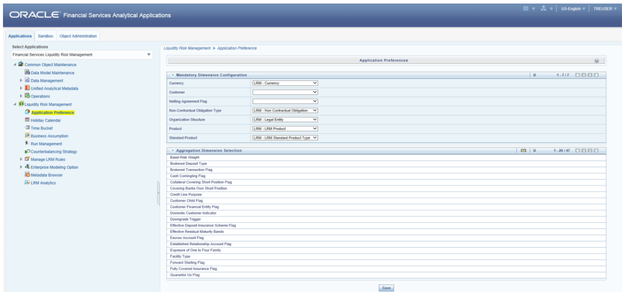
Figure 4 Application Preferences
